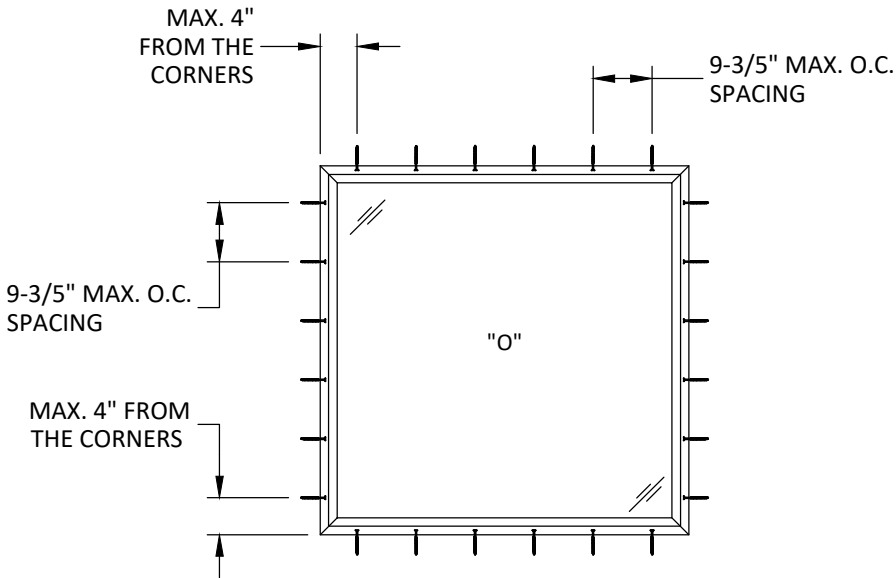
ANCHOR LAYOUT THROUGH FRAME INSTALLATION
