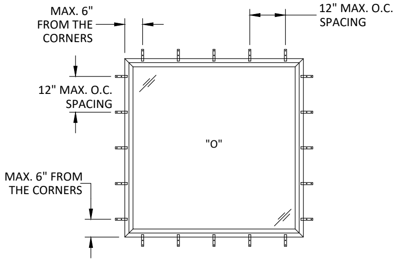
ANCHOR LAYOUT STRAP INSTALLATION
